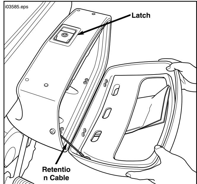
Figure 16. Saddlebag Lid Compartment
